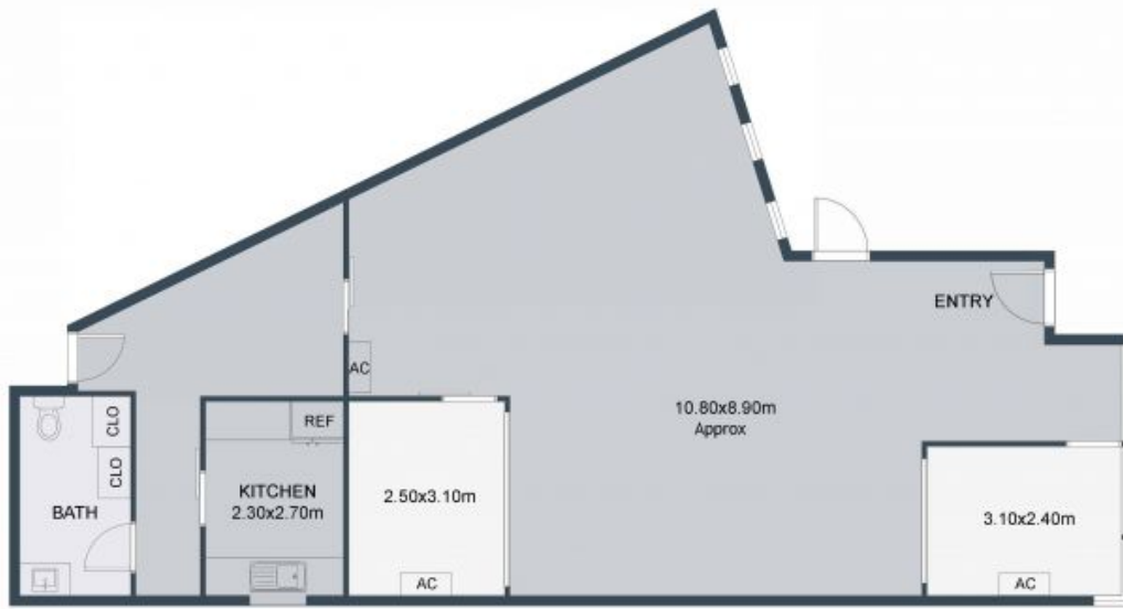
FLOOR PLAN
